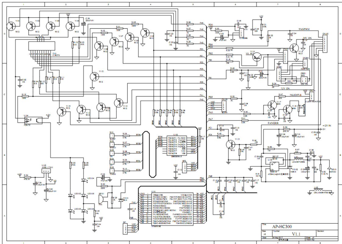
Control PCB
