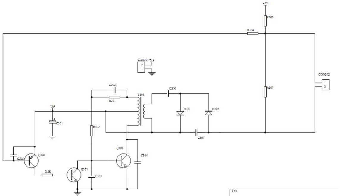
High-voltage part Circuit diagram
