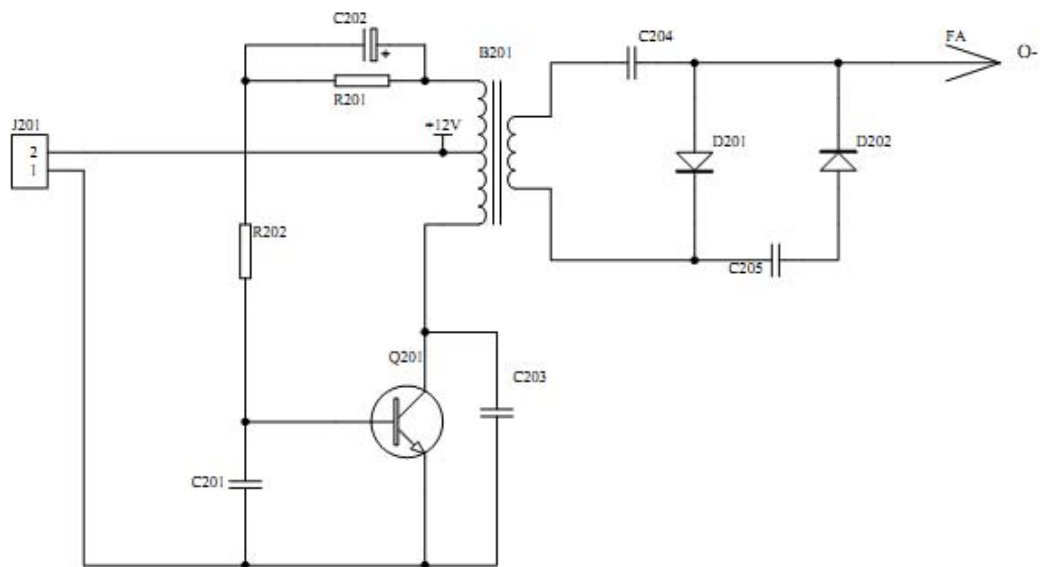
High-voltage part Circuit diagram
